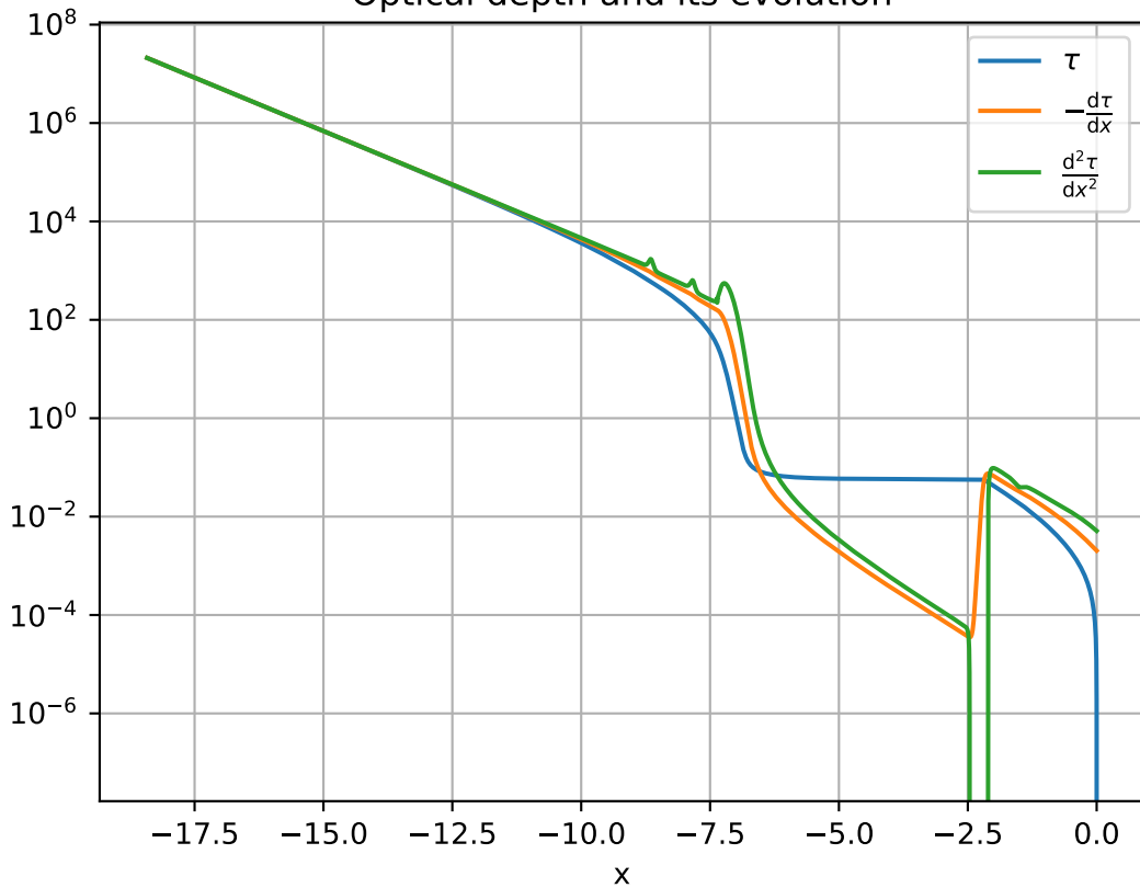
Optical depth and its evolution
